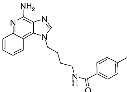
N -[4-(4-amino-1 H -imidazo[4,5- c ]quinolin-1-yl)butyl]-4-methylbenzamide;
